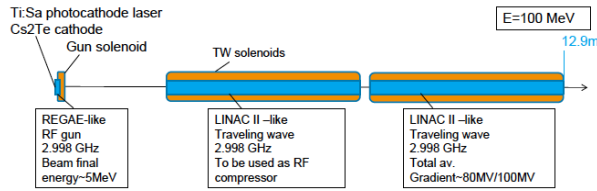
Figure 1: Layout of the ARES accelerator in the first stage of the experiment.
