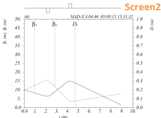
Figure 4: Example of simple beam optics for the bunch length measurement, delivering 90 degree of phase advance in the vertical plane between the centre of the transverse deflecting cavity and a screen located on the straight line.
