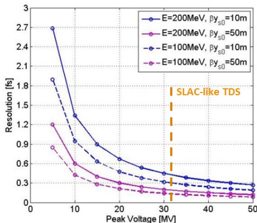
Figure 5: Resolution of the bunch length measurement (cfr. references [16, 17]) for different energies of the electron beam and vertical \beta_{y,s0} Twiss parameter in the centre of the TDS as a function of the deflecting Voltage of the cavity. A phase advance of 90 degrees in the vertical plane between the centre of the TDS and the screen is assumed.
