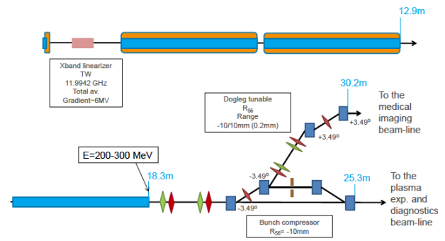
Figure 2: Layout of the ARES accelerator in the second stage of the experiment.
