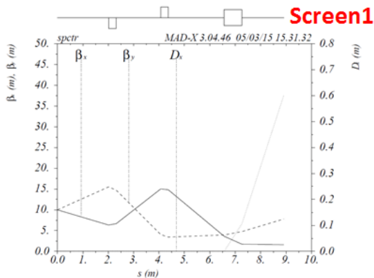
Figure 3: Example of simple beam optics for the longitudinal phase space measurement, delivering 90 degree of phase advance in the vertical plane between the centre of the transverse deflecting cavity and a screen located on a secondary line. The vertical Twiss parameter in the centre of the TDS ( \beta_{y,s0} ), located at z=0 , is 10 m. The dipole represented in the sketch has an angle of 17.5 degrees with respect to the main line.
