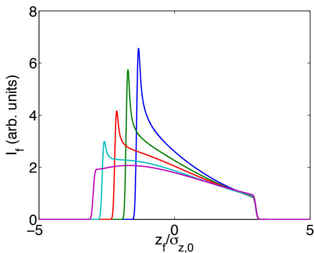
Figure 1: Current profiles analytically obtained from Eq. 3 for b_f = 0.7 and a_f = 2.0, 2.25, 2.5, 2.75, and 3.0 corresponding to decreasing current from blue to magenta traces (we took \sigma_u = 0.05 ).
