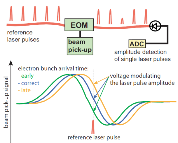
Figure 2: Principle of the arrival time measurement. The laser pulses are modulated by the EOM which is driven by the RF signal from the pickup. Arrival time changes of the electron bunch cause different modulation voltage at the laser pulse arrival time. [9]
